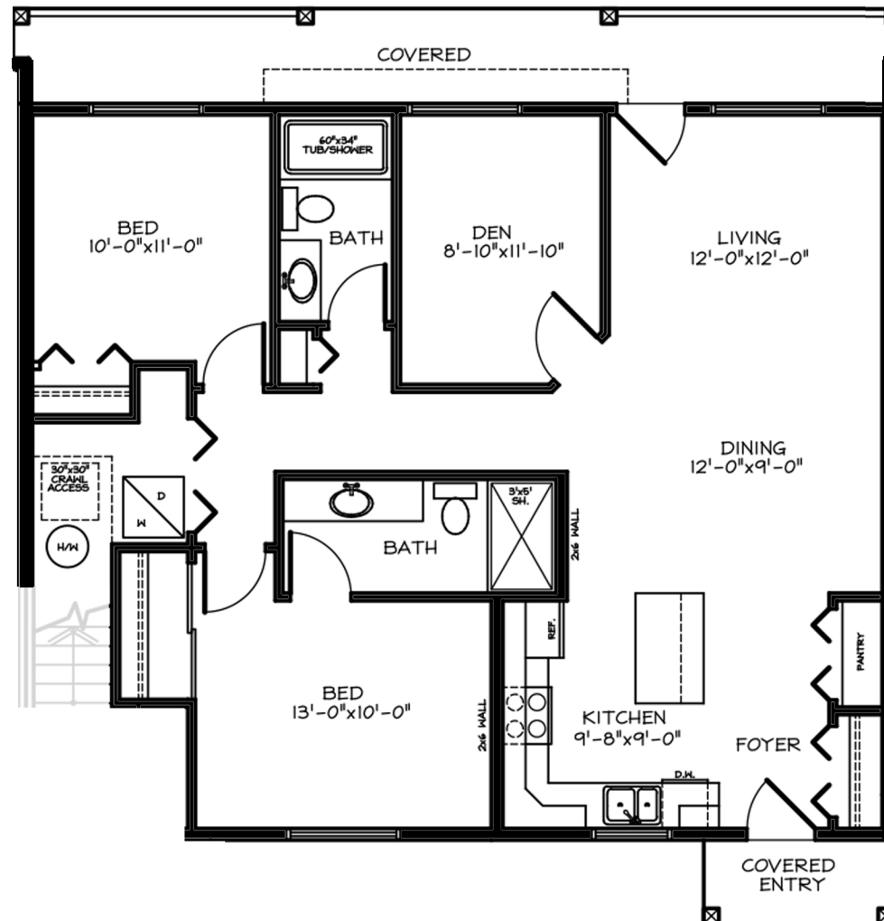
MAIN FLOOR PLAN 'B' 1161 SQ. FT. TOTAL
