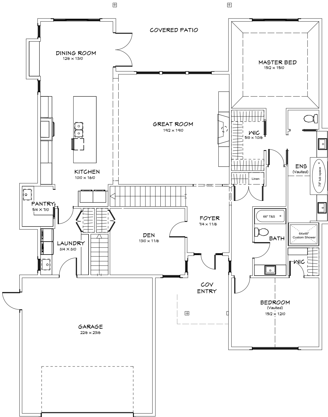
MAIN LEVEL - 2,265 SQ.FT.
