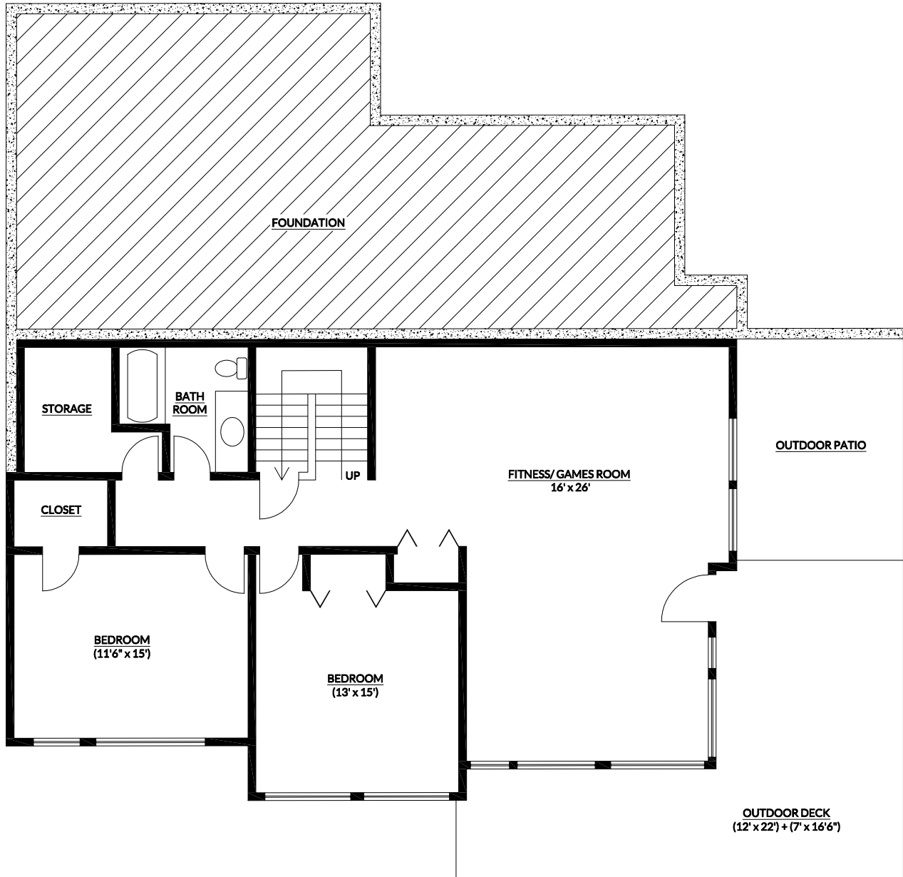
BASEMENT FLOOR PLAN 1090 SQFT LIVING AREA (UNFINISHED)
