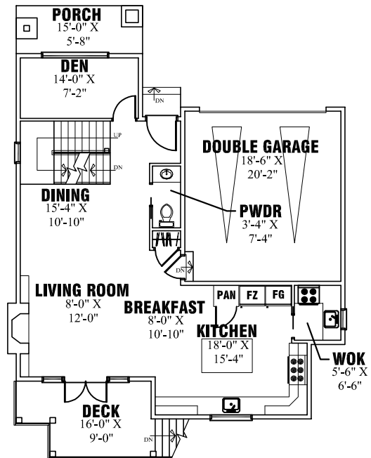
MAIN FLOOR PLAN 1038.1667 SQ.FT.
