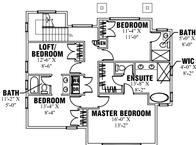
UPPER FLOOR PLAN 1111.4583 SQ.FT.
