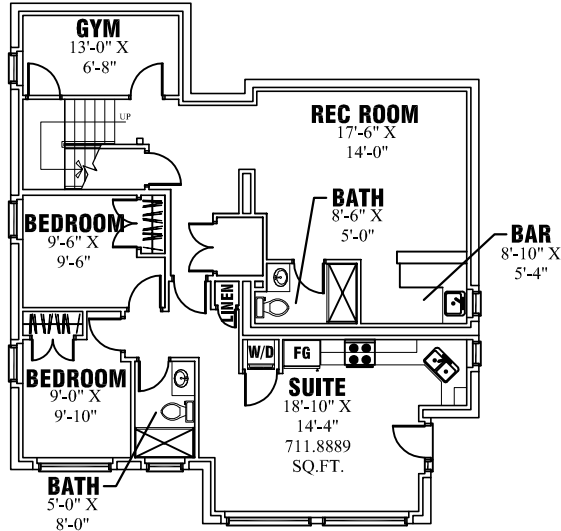
BASEMENT FLOOR PLAN 1425.4167 SQ.FT.
