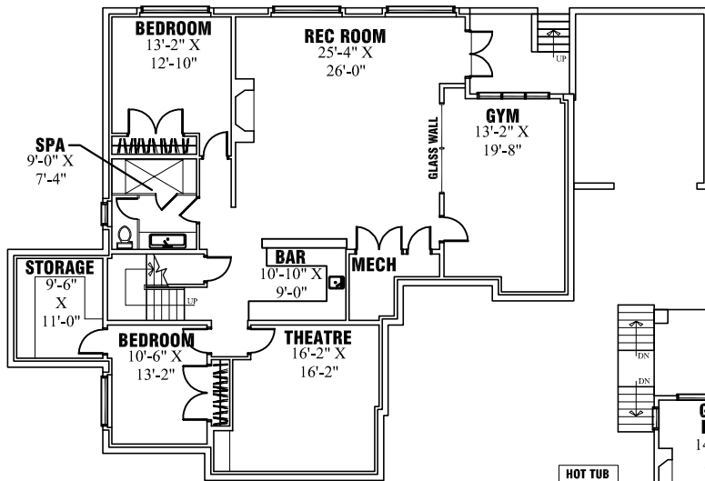
BASEMENT FLOOR PLAN 2284.0556 SQ.FT.
