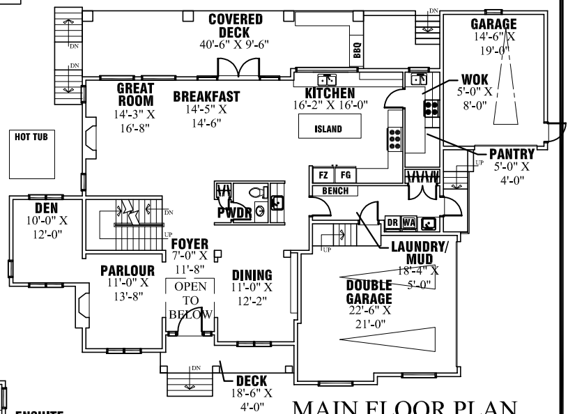
MAIN FLOOR PLAN 1842.2222 SQ.FT.
