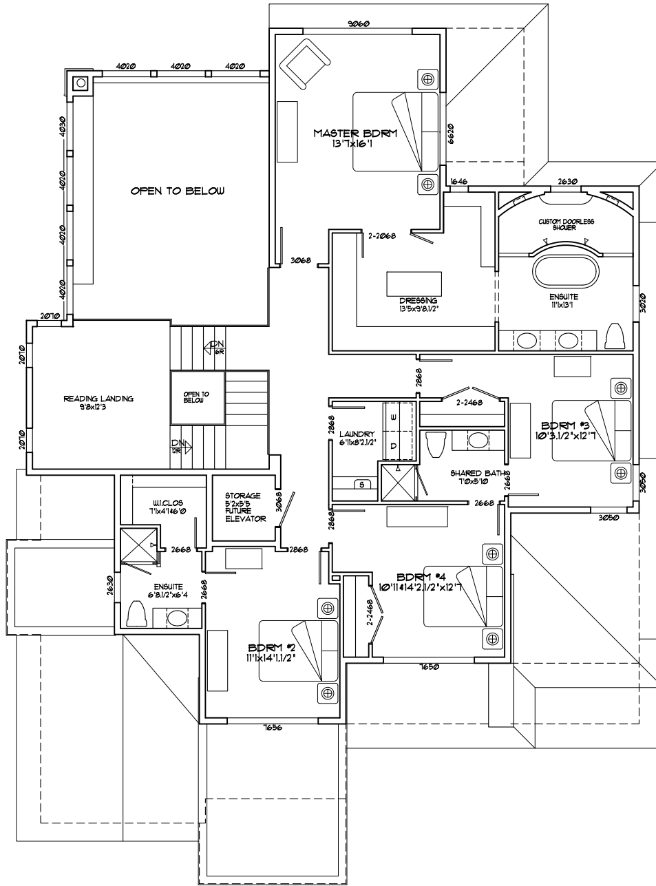
UPPER FLOOR PLAN 1639.86 SQ.FT. PLUS STAIRS & OPEN TO BELOW
