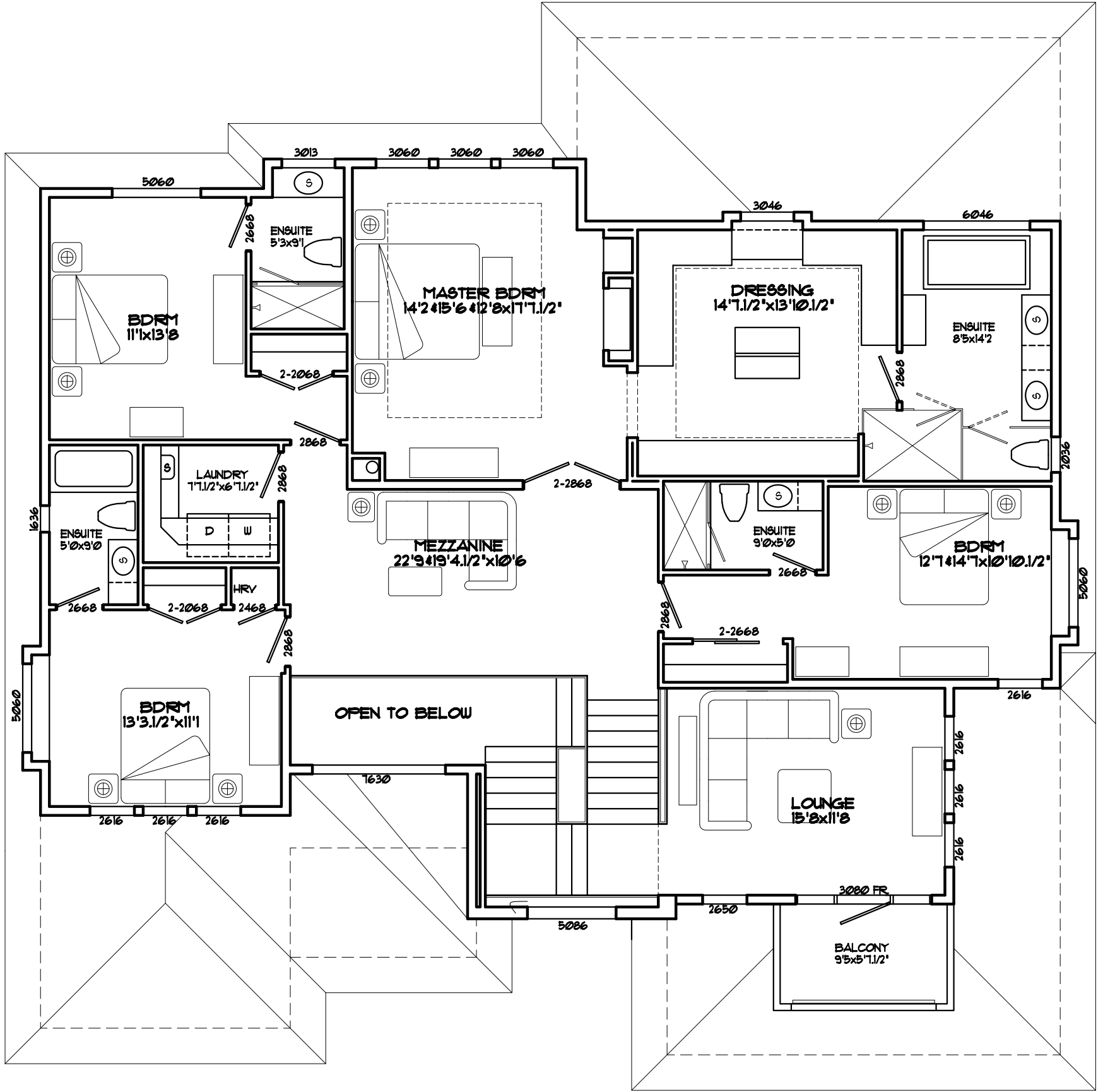
UPPER FLOOR PLAN 1,891.49 SQ.FT. PLUS STAIRS & OPEN TO BELOW
