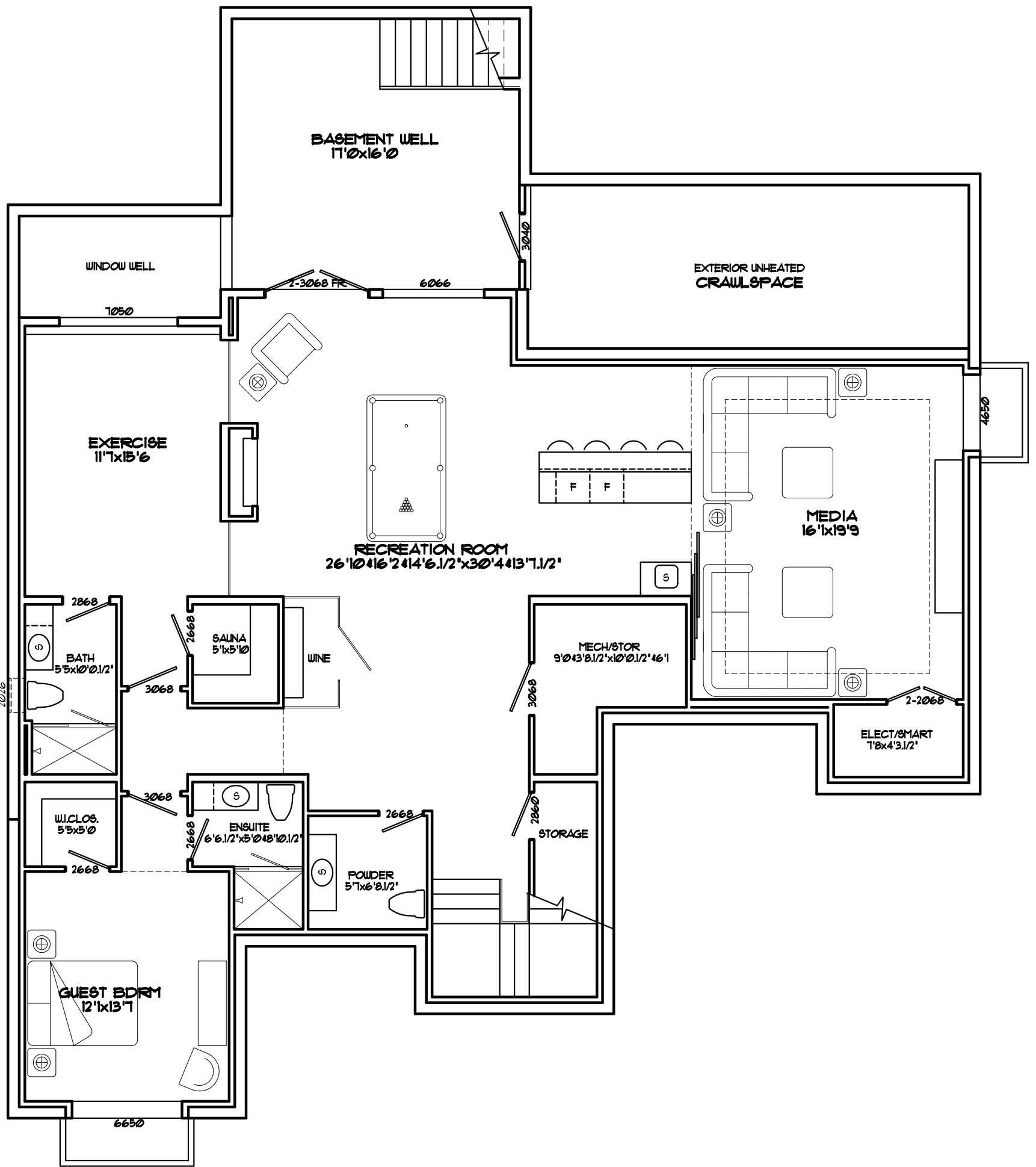
BASEMENT PLAN 2,064.00 SQ.FT.
