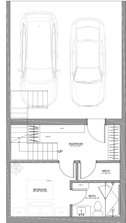
BASEMENT
