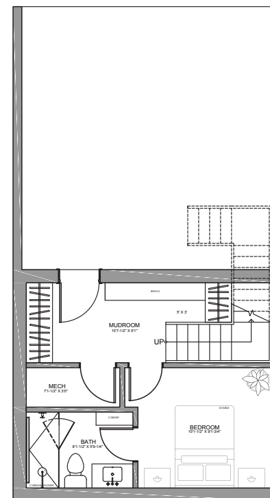
BASEMENT
